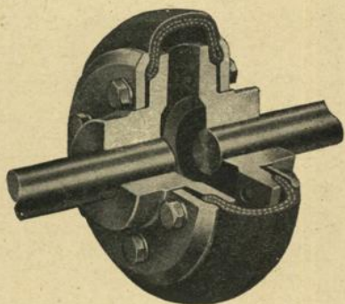
PERIFLEX-Wellenkupplung
