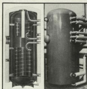
▲ Boiler 120-1000 l
